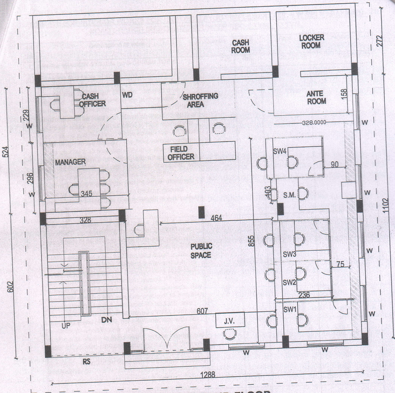
MARAKKADA BRANCH -GROUND FLOOR (RENOVATION)-Dwg no.1 dt.10.10.24
